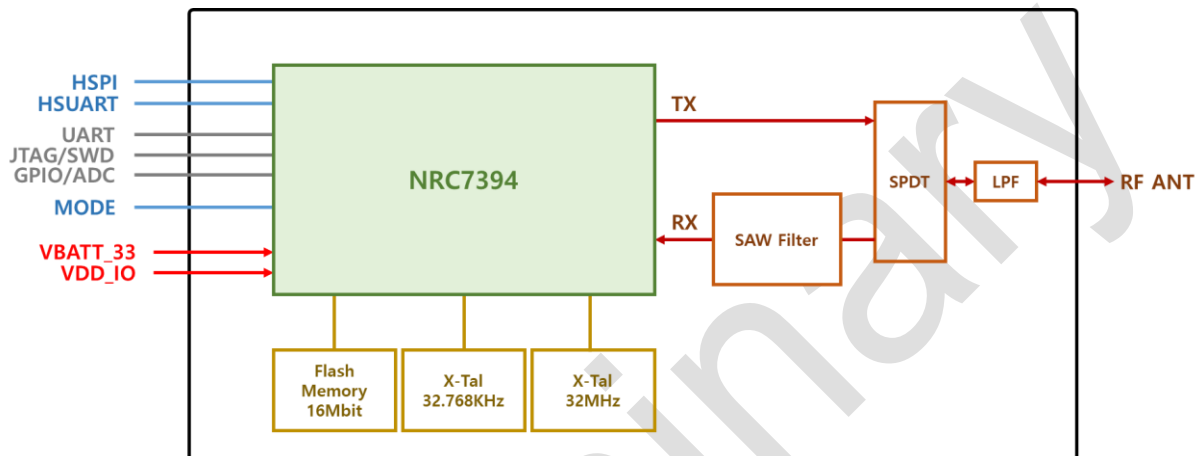
Figure 2-1: Block Diagram
